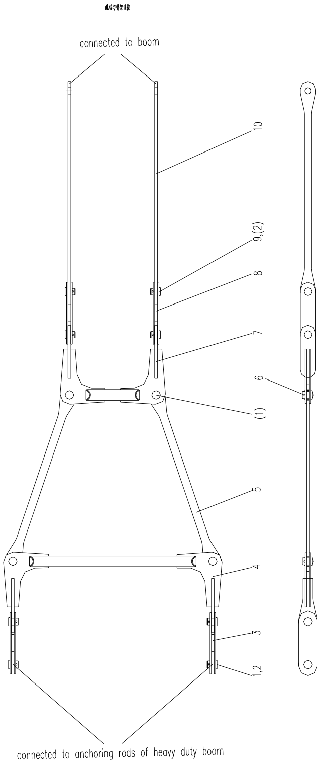
1. length of anchoring rods of heavy duty boom
